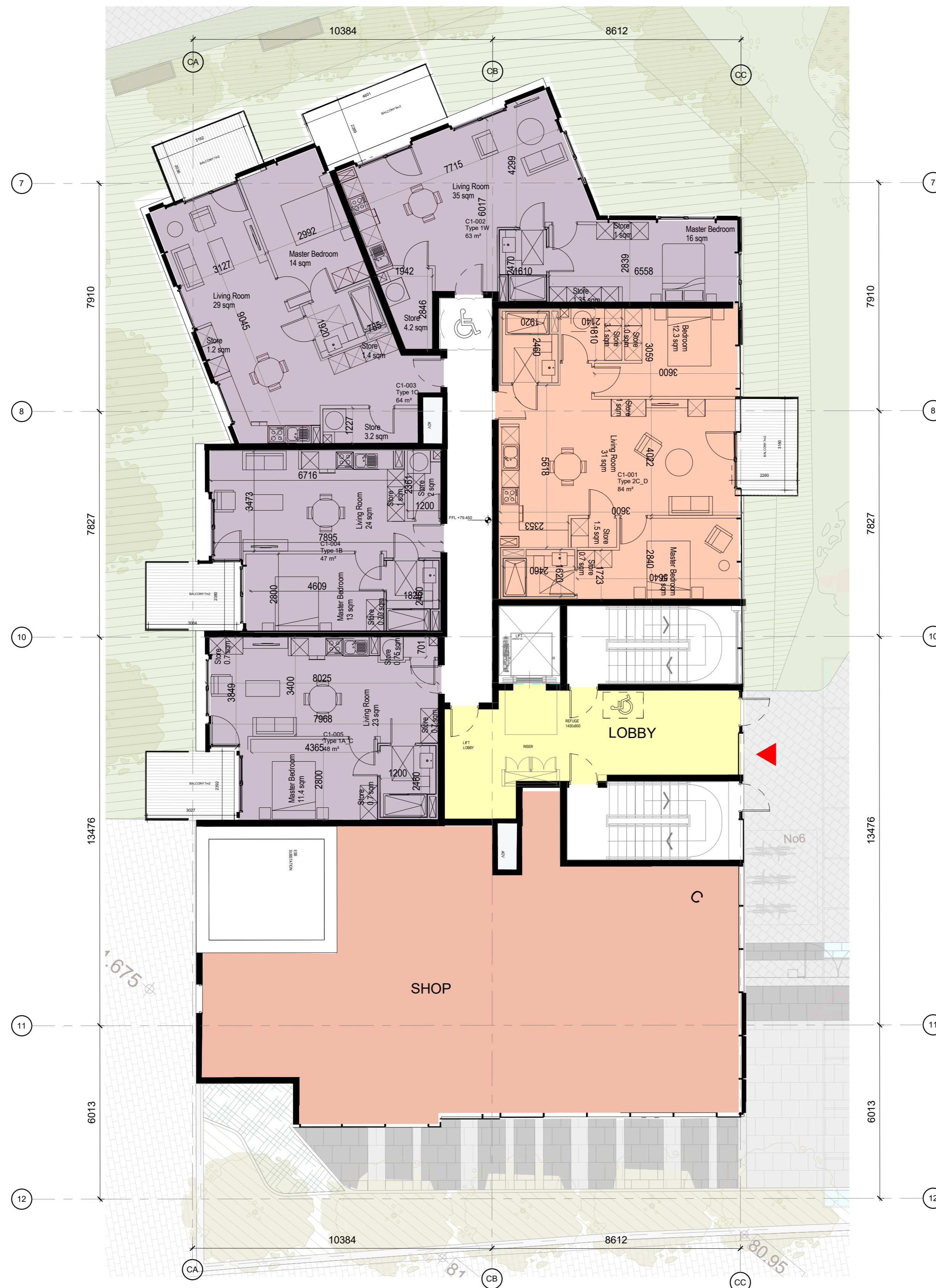
1 00 FFL GA Part V Block C 1 : 100
